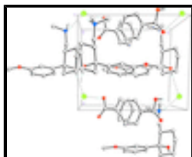
Fig. 2. Packing diagram of the title co-crystal salt viewed down the c axis. Dashed lines indicate weak O—H...Cl and N—H...Cl intermolecular interactions forming a supramolecular 2-D chain network along the a axis.
